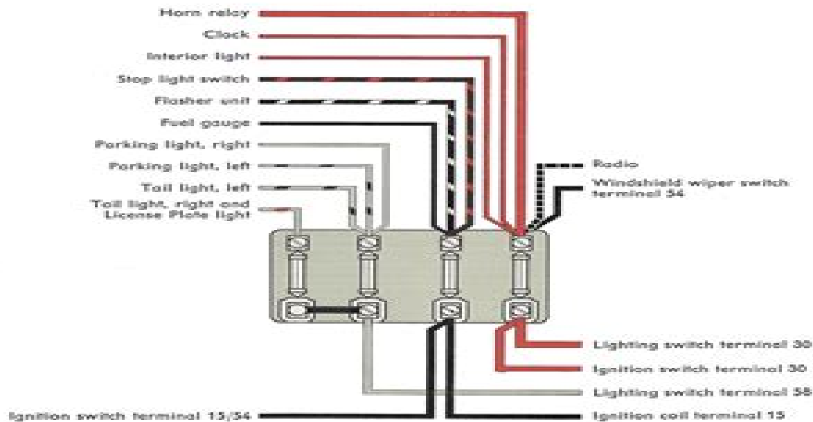
Fuse box on the back of the instrument panel
